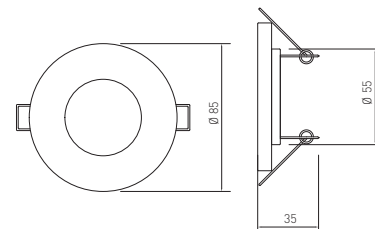
MR16
